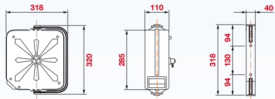
OVERALL DIMENSIONS
